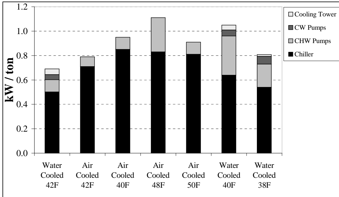
Figure 7. Chilled Water System Comparison
