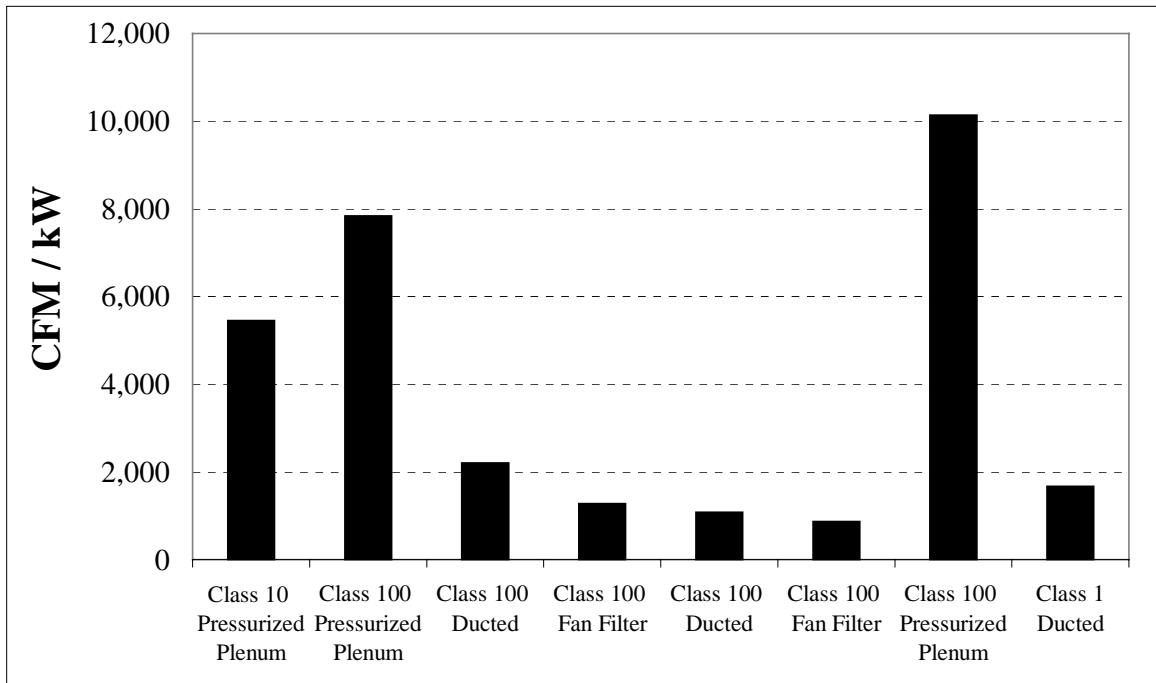
Figure 3. Cleanroom Air Recirculation System Efficiency
