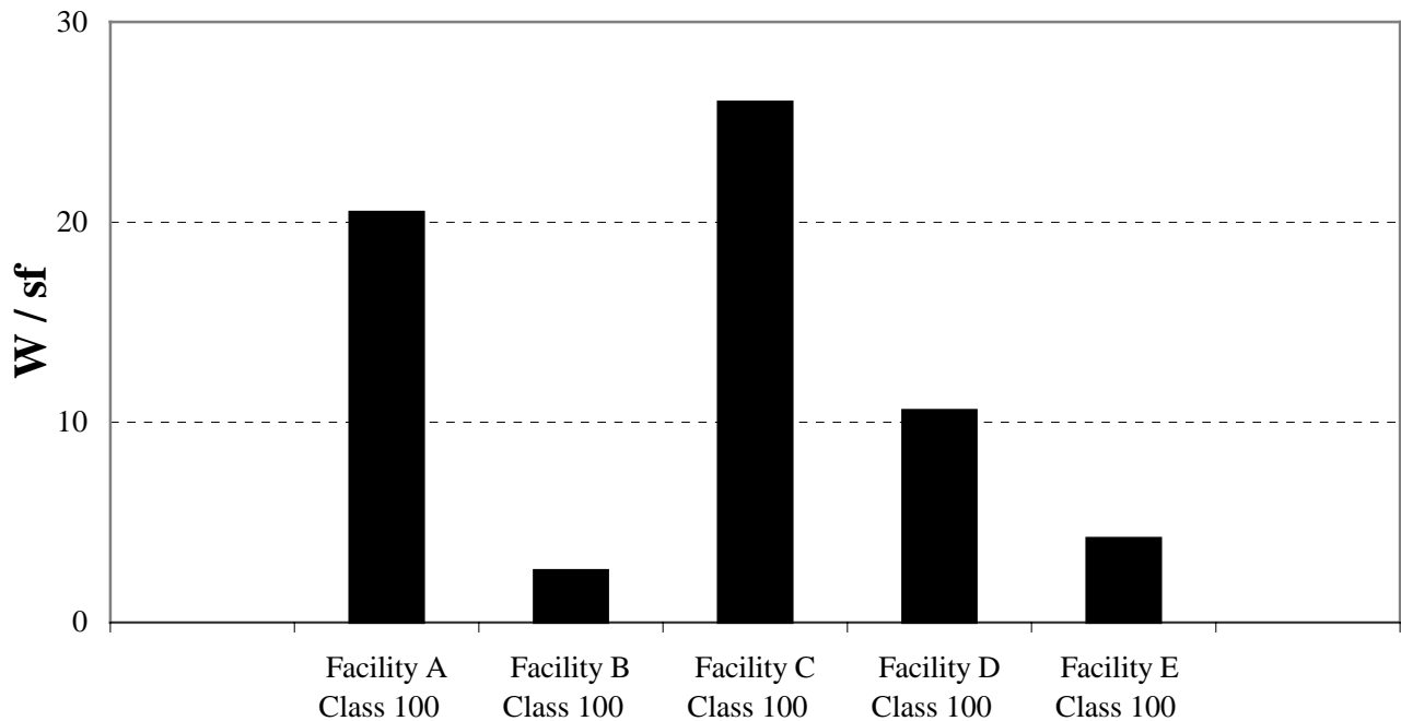
Figure 8 Class 100 Cleanroom Intensity Variation
